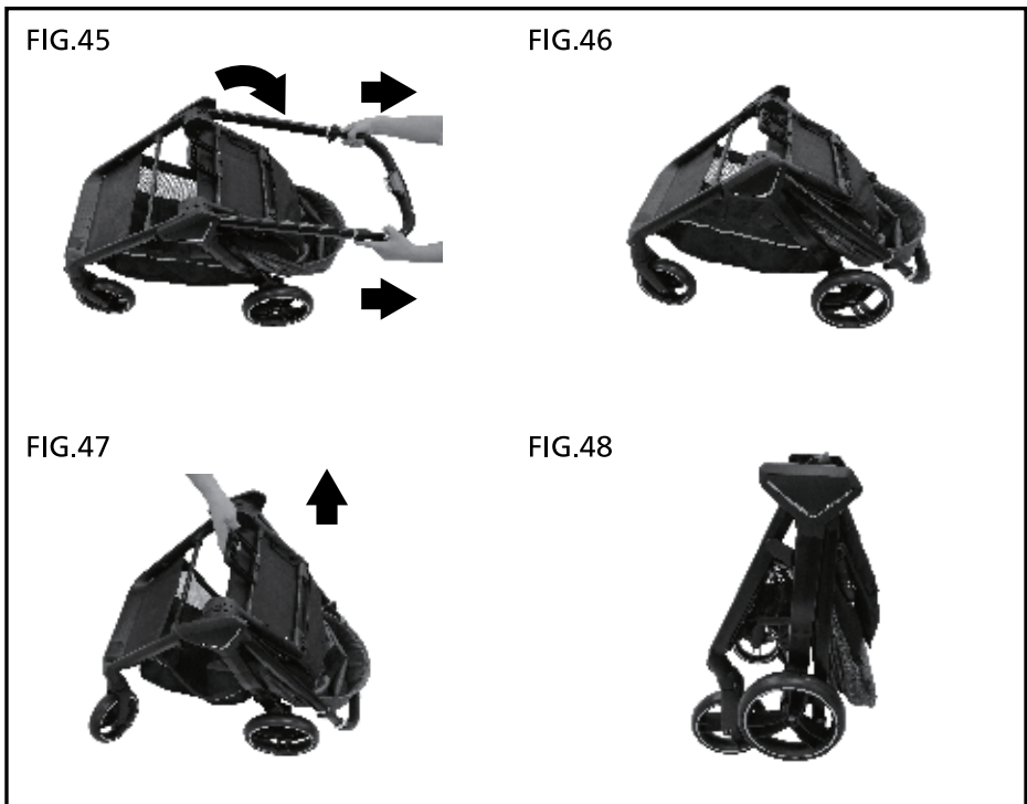
Pull the folding levers on both sides of the handle bar and push down the handle bar to fold the stroller.(FIG.45&46&47&48)
