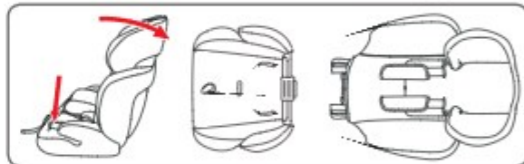
Backrest removal: Disconnect the the backrest and base, take out the backrest's hook from the rubber band of the seat cover of the base, Separate the backrest from the base, and the base can used with Group 3 modes.
